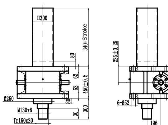
Mounting View
