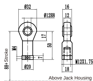
Spherical Hinge
