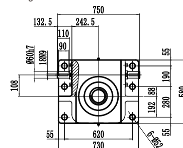
Mounting View
