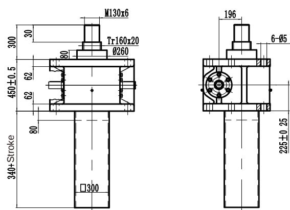
Installation diagram
