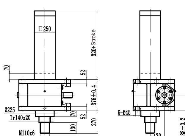
Mounting View
