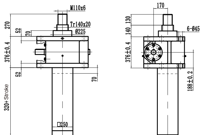
Installation diagram
