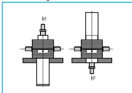
Installation diagram
