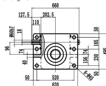
Mounting View
