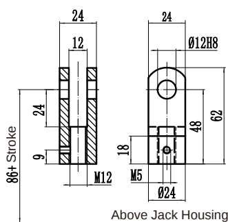
Forked Head
